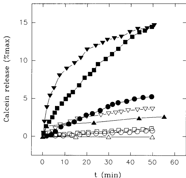
FIGURE 5 Calcein release (% of max) as a function of time in the absence (empty symbols) and in the presence (filled symbols) of PEG (20% w/v). \circ, \bullet , PLE at T = 25^\circ\text{C} ; \triangle, \blacktriangle , PLE/P2, 1:2 m.r. at T = 25^\circ\text{C} ; \square, \blacksquare , PLE/PC, 1:2 m.r. at T = 25^\circ\text{C} ; \nabla, \blacktriangledown , PLE at T = 60^\circ\text{C} .
