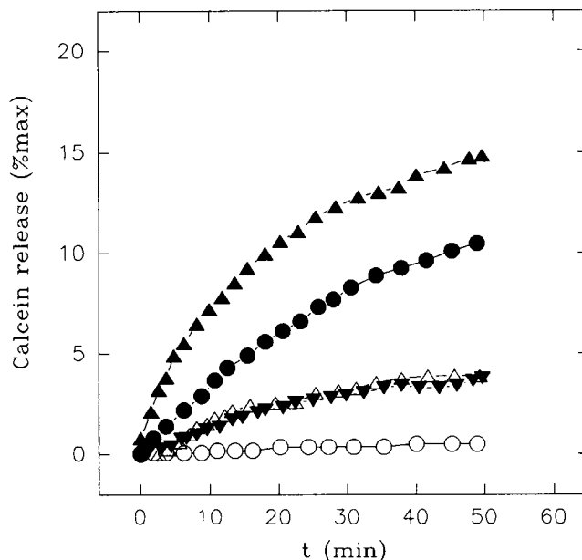
FIGURE 6 Calcein release (% of max) as a function of time for P2 vesicles in the absence (empty symbols) and in the presence (filled symbols) of destabilizing agents. \triangle, \blacktriangle, \nabla , T = 60^\circ\text{C} ; \circ, \bullet , T = 25^\circ\text{C} . \blacktriangle , in the presence of 20% w/v PEG; \nabla , in the presence of 15 mM \text{Ca}^{2+} ; \bullet , in the presence of 20% w/v PEG.
